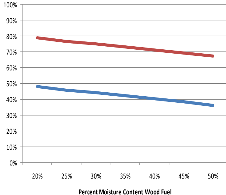
Thermal Efficiency and Moisture Content for Park Falls Cogen Plant Compared to a Utility
